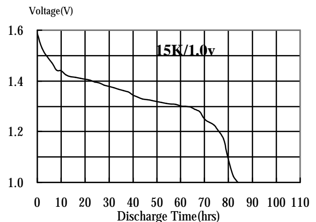
Typical Discharge characteristics for Reference only at 20 \pm 2^\circ\text{C}
