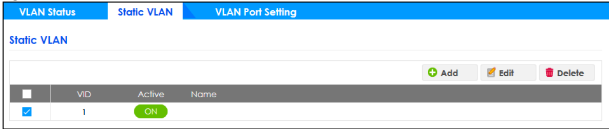
Figure 452 Switching > VLAN > Static VLAN
