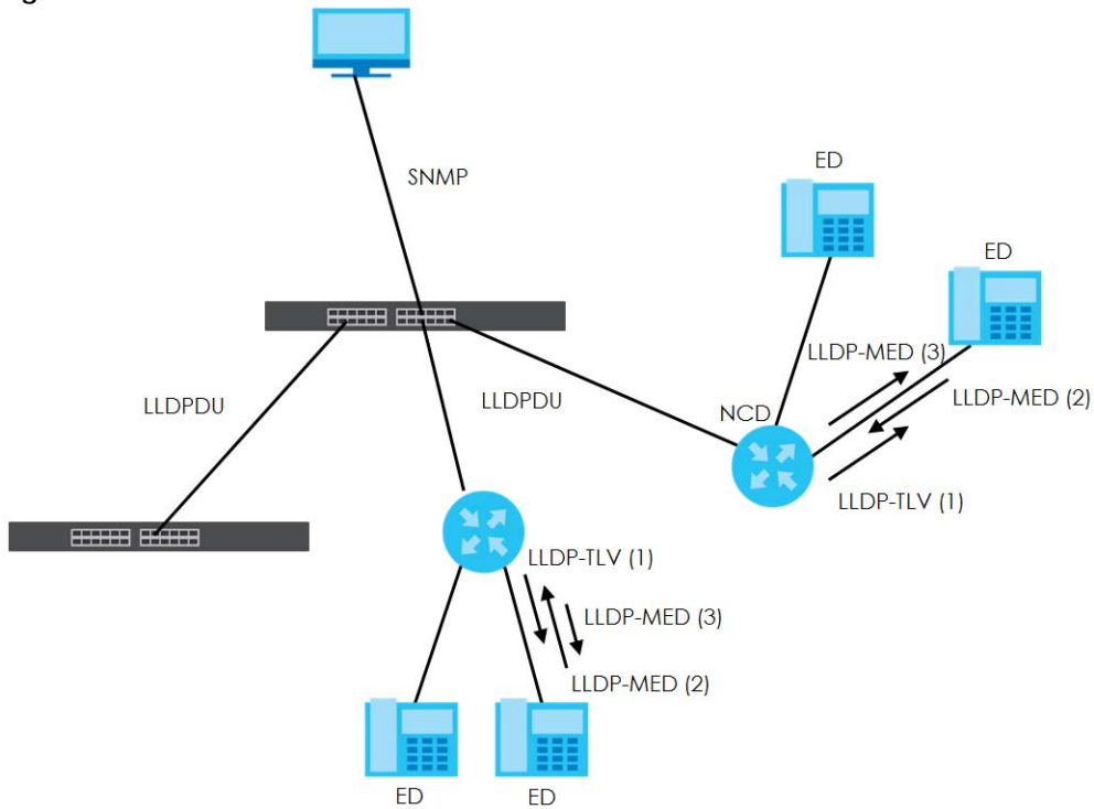
Figure 286 LLDP-MED Overview
