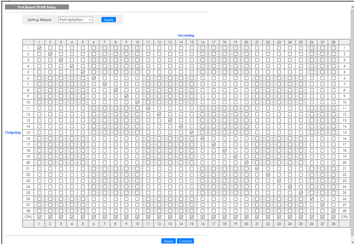
Figure 124 Advanced Application > VLAN: Port Based VLAN Setup (Port Isolation)
