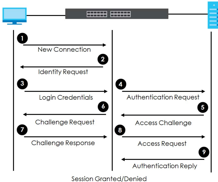
Figure 168 IEEE 802.1x Authentication Process
