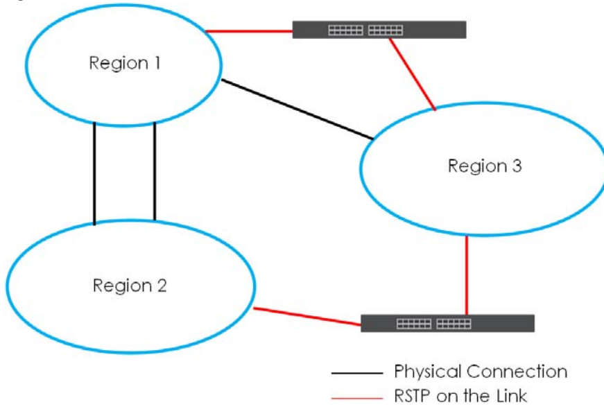
Figure 154 MSTP and Legacy RSTP Network Example
